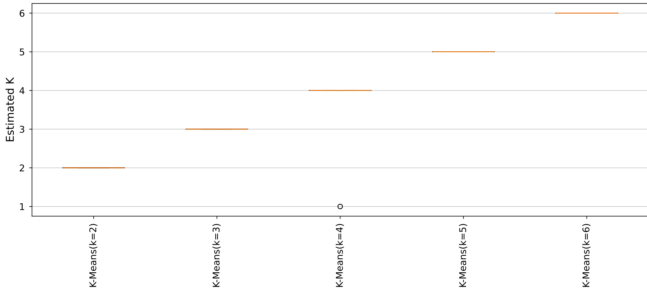
YARA Rules Estimated K Distribution (Cluster29_Size6 dataset)
